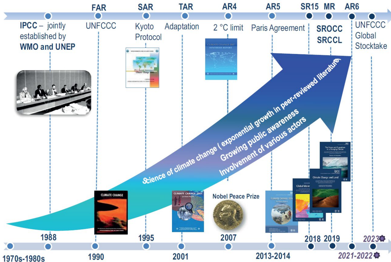
Aus: IPCC, 2017 – The IPCC and the Sixth Assessment Report
