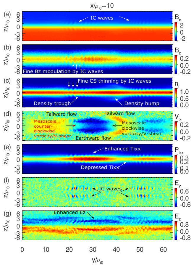
Figure 4. Results from the same 3D Particle-In-Cell simulation as in Figure 2 in the yz plane at x/\rho_{i0} = 10 : B_x (a) and B_z (b) magnetic field components, ion density (c), ion velocity V_{ix} component (d), P_{xx} ion pressure tensor component (e), E_y (f) and E_z (g) electric field component. The coordinates are expressed in \rho_{i0} —the ion gyroradius in the asymptotic lobe B_0 field.
