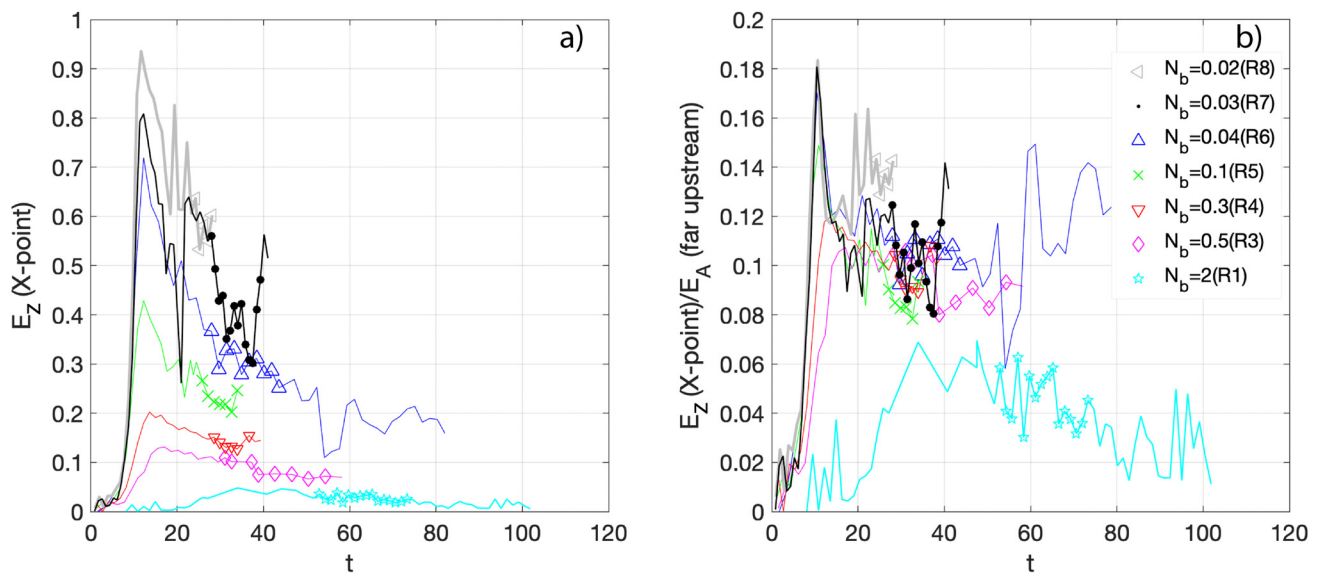
FIG. 3. (a) Un-normalized reconnection rate (electric field E_z at the main X-line). (b) Microscopic ion reconnection rate \epsilon_r = E_z/E_A^{(up)} , for all runs. In each line, the symbols mark moments chosen for quasi-steady study.
