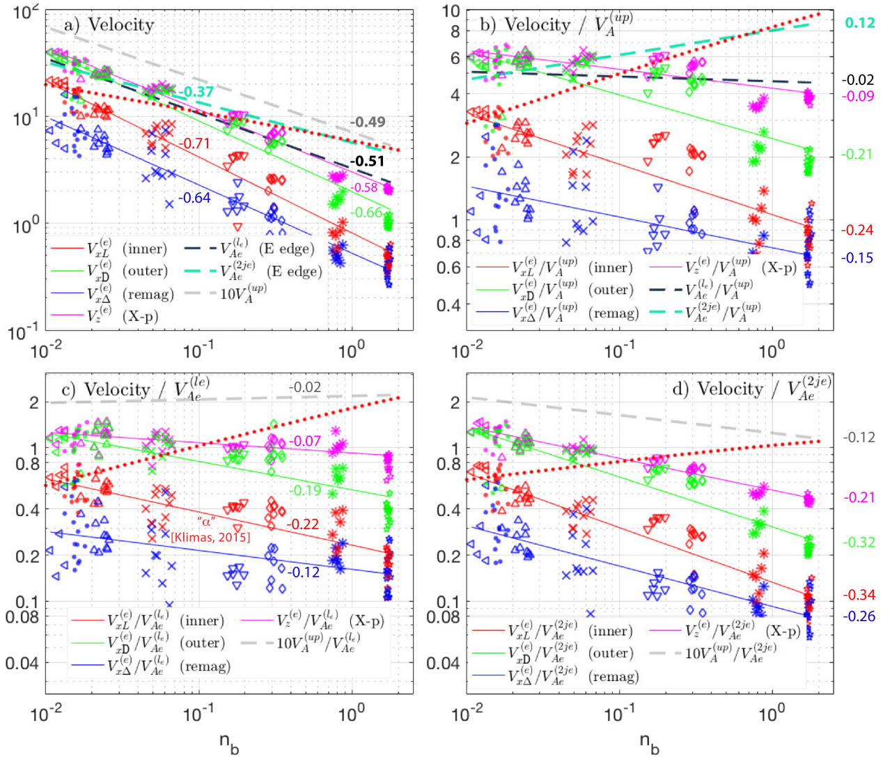
FIG. 8. Characteristic EDR velocities combined for all runs: (a) un-normalized. (b) Velocities / V_A^{(up)} . (c) Velocities / V_{Ae}^{(le)} . Notably, the ratio V_{xL}^{(e)}/V_{Ae}^{(le)} is denoted 52 as \alpha and has a significant trend with density, \alpha \sim n_b^{-0.22} . (d) Velocities / V_{Ae}^{(2je)} . Respective power law fits are shown with numbers.
