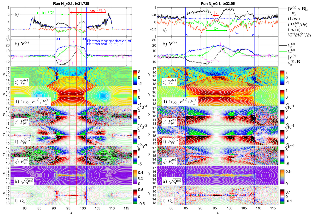
FIG. 1. (a) Ohm's law terms. (b) Electron velocities and the x component of the \mathbf{E} \times \mathbf{B} drift speed ( V_x^{(e)} ). (c) V_y^{(e)} . (d) \log_{10} P_{\parallel}^{(e)} / P_{\perp}^{(e)} . (e) P_{yz}^{(e)} . (f) Gyrotropic part of P_{yz}^{(e)} , given by P_{yz}^{(e)G} = (P_{\perp}^{(e)} \mathbf{I} + (P_{\parallel}^{(e)} - P_{\perp}^{(e)}) \mathbf{b}\mathbf{b})_{yz} , where \mathbf{b} = \mathbf{B}/|\mathbf{B}| is the magnetic field direction. (g) Rotated component \tilde{P}_{yz}^{(e)} . (h) Electron nongyrotropy measure \sqrt{Q^{(e)}} . (i) Electron dissipation measure D_e' . Plots are shown for two selected time slices, before ( t=21.728 ) and after ( t=33.95 ) the quasi-steady EDR regime is reached. Definitions of inner EDR, outer EDR, and electron braking (remagnetization) region are shown in left panels. Length measures L_e , D_e , and \Delta_e are shown in right panels.
