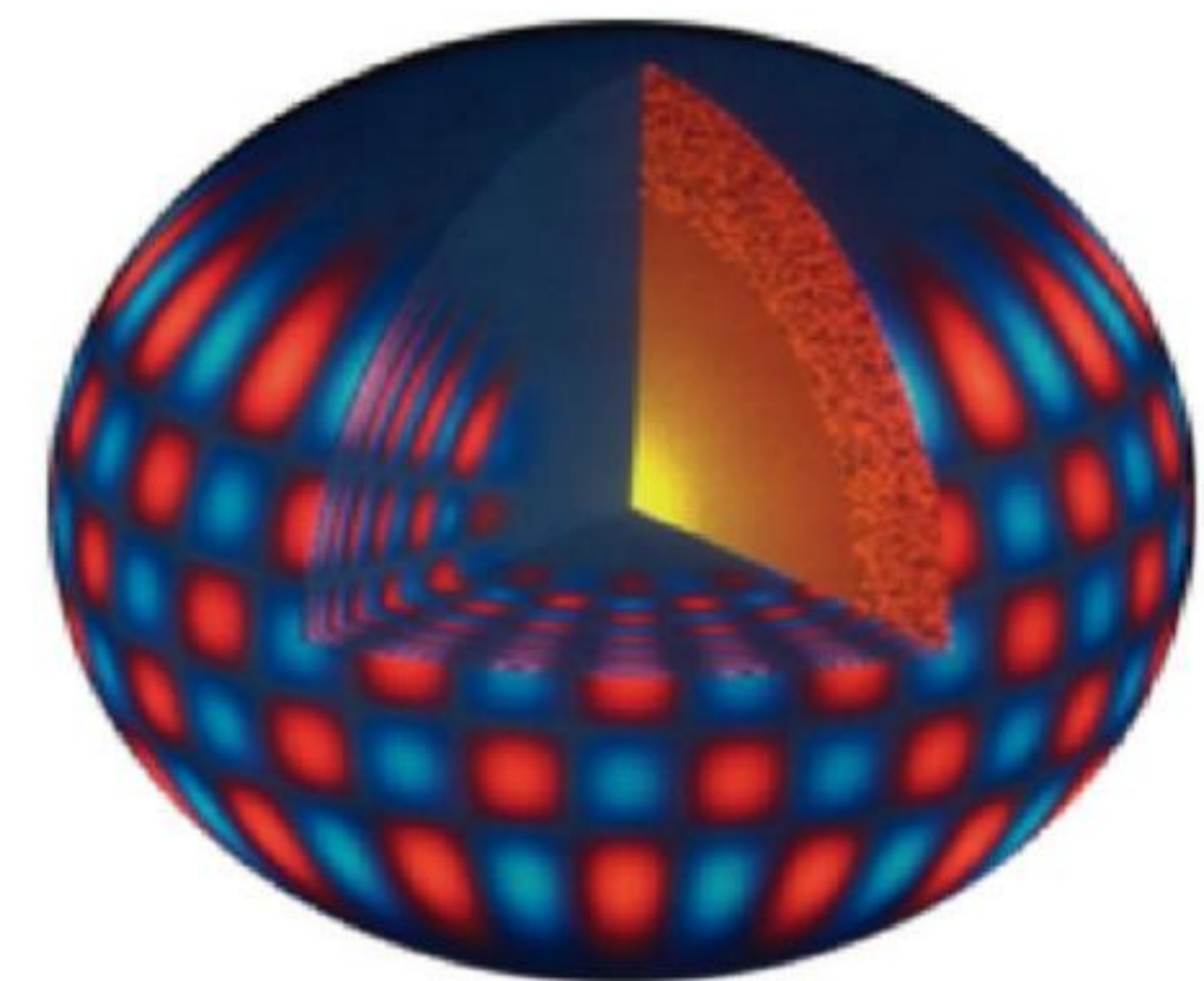
Oscillations (p-modes)
