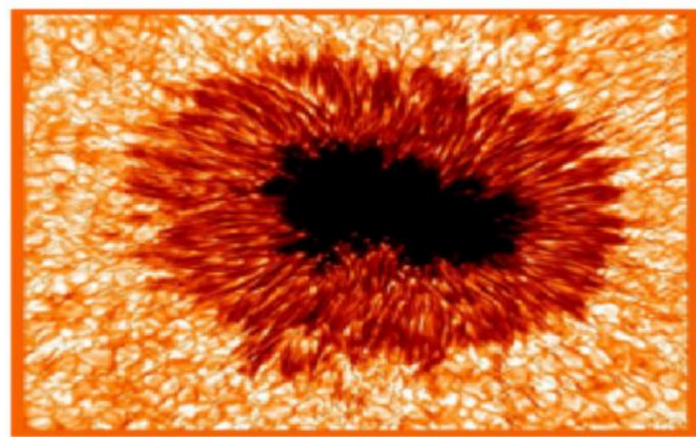
Magnetic activity (spots, plages, ..)
