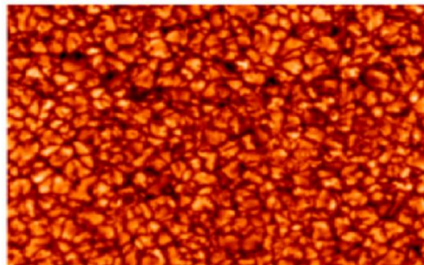
Convective phenomena (Granulation, ..)
