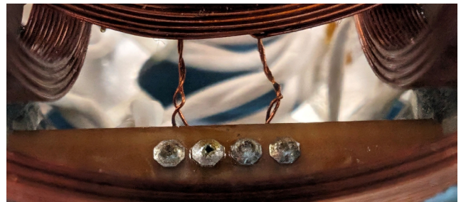
BFG EFM sensors after vibration test (©OeAW/IWF/Valavanoglou).
