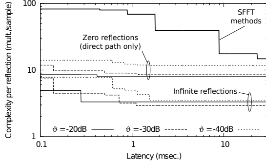
Figure 5. Latency-complexity trade-offs for different values of \vartheta and number of reflections.
