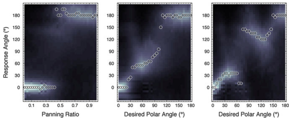
Fig. 22 Predictions for VBAP applied to various surround-sound systems. Left 5.1 setup, panning between the loudspeakers L and LS. Center 10.2 DSX setup panning from L, polar angle of 0^\circ , via LH2, 55^\circ , to LS, 180^\circ . Right 9.1 Auro-3D setup panning from L, 0^\circ , via LH1, 34^\circ , and LSH, 121^\circ , to LS, 180^\circ . Desired polar angle Continuous scale representing VBAP across pair-wise contributing loudspeakers. All other conventions are as in Fig. 18
