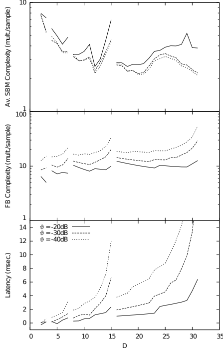
Figure 4. Average complexity per HRTF of the SBMs (top), complexity of either the analysis or the synthesis FB (center) and implementation latency (bottom) vs. down-sampling factor D , for various FB prototype energy leakage thresholds \vartheta .
