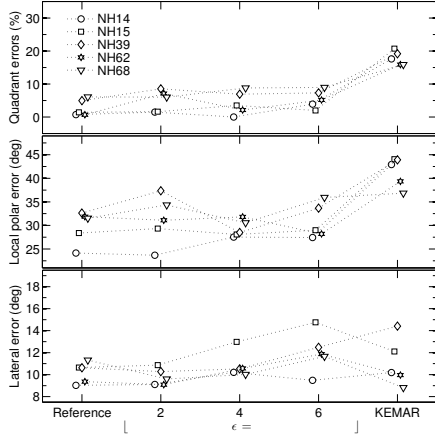
Figure 3. Listener-specific sagittal-plane localization performance obtained in psychoacoustic experiments. Note the robustness of each listener's performance across various \epsilon .
