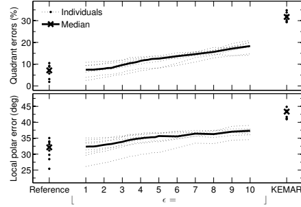
Figure 2. Predicted sagittal-plane localization performance as a function of approximation tolerance \epsilon . Notice that performance for \epsilon = 1 is close to the one for individually measured DTFs (Reference), whereas performance for \epsilon = 10 remains better than for non-individualized DTFs (KEMAR).
