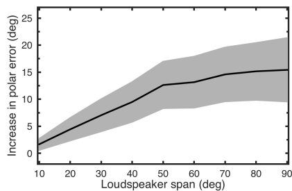
Fig. 7. Increase in polar error as a function of loudspeaker span in the median plane with amplitude ratio \Delta L = 0 . Increase in polar defined as for Fig. 5; mean \pm 1 SD across listeners. Note the systematic increase in polar error with increasing loudspeaker span.
