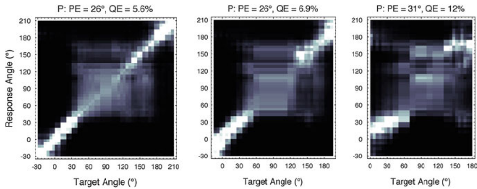
Fig. 19 Predictions for different loudspeaker spans and NH12. Left Span of 0^\circ , single-loudspeaker synthesis, baseline condition. Center Span of 30^\circ . Right Span of 60^\circ . All other conventions are as in Fig. 8
